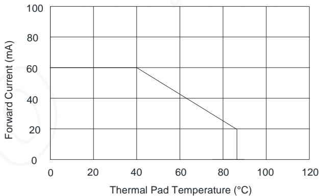
Thermal Pad Temperature vs. Forward Current
